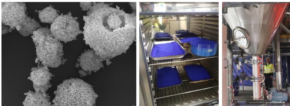
Figure 1: MOFs (HKUST-1) beads of 80 \mu\text{m} in diameter prepared by spray-drying process
